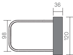
Type A Straight Bar
