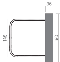
Type AA Double Straight Bars
