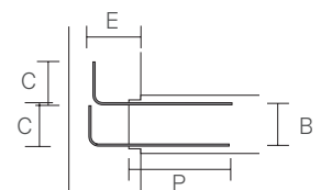
Type LL Cog Bars
