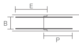
Type AA Double Straight Bars
